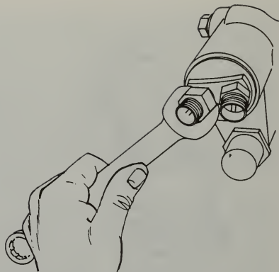
FIGURE 6-19. Removing oil temperature bulb.
